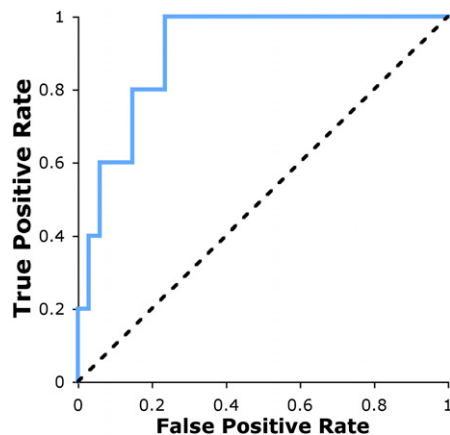
Fig. S2. Receiver operating characteristic (ROC) curve for the digital PCR assay using the endomyocardial biopsy grade \geq 3A-2R as an indicator of true positives. All sampled data points (39 total) for patients 7–13 are included. The first time point for patient 10 occurred during an antibody-mediated rejection episode and is included in this curve as a true positive. The area under the curve is 0.906.
