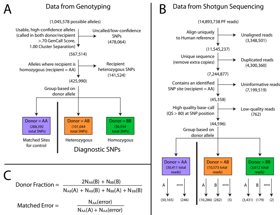
Fig. S3. Scheme of workflow for determining usable SNP alleles and calculating donor fraction from sequencing. (A) Data from genotyping chip (representative numbers provided for patient 14) are first filtered as indicated, removing alleles with no calls as well as low-confidence alleles (with low GenCall or cluster separation scores as reported by Illumina). Homozygous recipient SNPs are then selected (recipient = AA), and the donor SNP information leads to binning into three categories depending on whether the donor is a full match to the recipient (=AA), or has a heterozygous (=AB) or homozygous (=BB) allele difference from the recipient. The first grouping offers a matched control for determining base-line errors, whereas the latter two groupings contain donor-specific variations that can be used diagnostically to calculate donor fraction. (B) Data from shotgun sequencing (representative numbers provided for month 18 sample for patient 14) are first filtered as indicated, on the basis of whether the reads aligned, were unique or duplicated, contained a relevant SNP site, and contained a high-quality base call at the SNP position. The remaining reads are then grouped into the same three classifications depending on whether the donor fully matches the recipient (=AA) or has a heterozygous (=AB) or homozygous (=BB) allele with a donor-specific variant. Within these groups, reads are then assigned as A, B, or an error (from any other base call at the indicated position). (C) Formulae used to calculate donor fraction and matched error fraction. Because the heterozygous donor case (=AB) results in only half as many identifiable donor reads as the expected number of donor molecules sampled, because half contribute to A calls, the formula uses twice the number of B reads from the heterozygous group. For the example data from the month 18 sample for patient 14, the calculated value for donor fraction is 0.0524 and for matched error is 0.0081.
