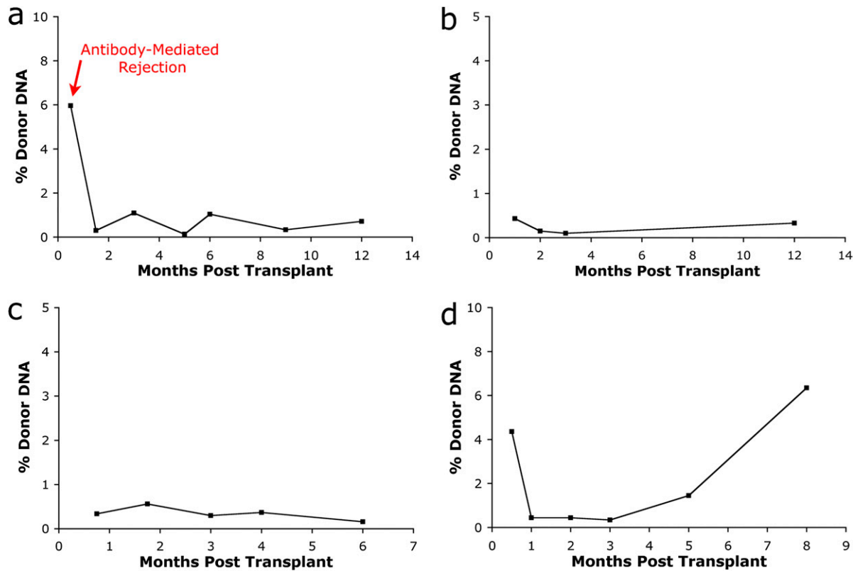
Fig. S1. Time course of chromosome Y levels (% donor DNA) in patients 10–13 (A–D) who had no endomyocardial biopsy-detected rejections in the sampled time periods. Patient 10 (A) was presensitized before transplant, with high levels of circulating HLA antibodies and likely had an antibody-mediated rejection during the first month after transplantation, which can explain the high initial response. The levels for this patient stabilize at or below ~1% for all subsequent time points. No documented medical events for patient 13 (D) are coincident with the higher signals at 0.5 and 8 mo.
